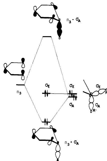
Figure 4. Hyperconjugation between the \pi_3 orbital of the pentadienylum moiety (left) and the \sigma orbital (right) of the axial bond -C-R' ; the \sigma orbital of the -C-R bond displays practically no overlap with the \pi system and consequently no hyperconjugation.
